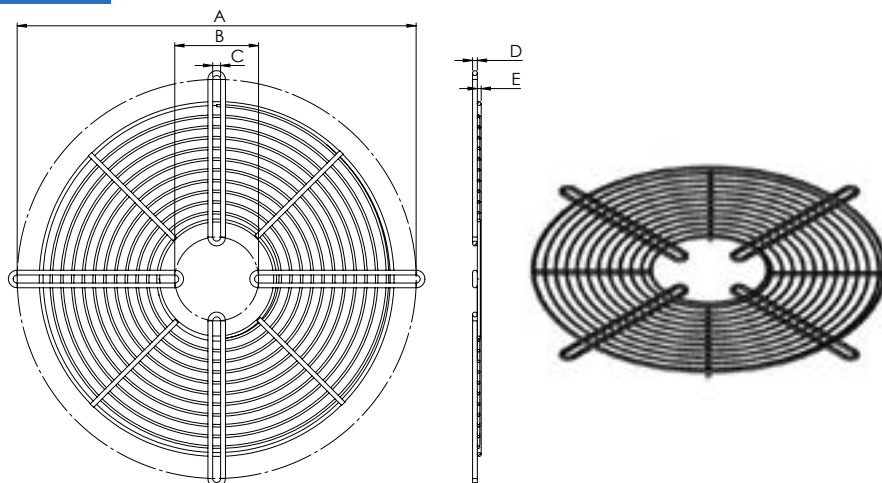
Dimensions (mm)
