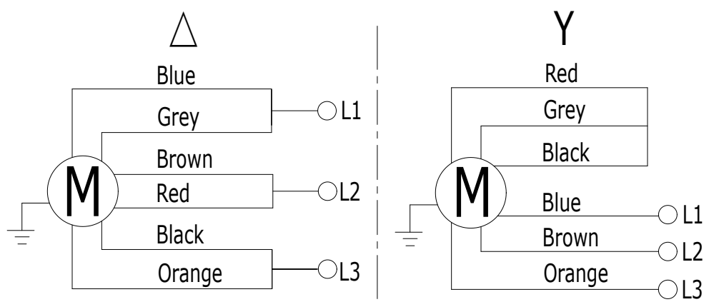
3-PHASE MOTOR WIRING DIAGRAM
