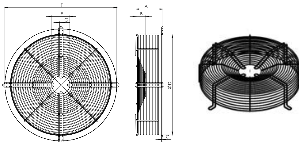
Dimensions (mm)
